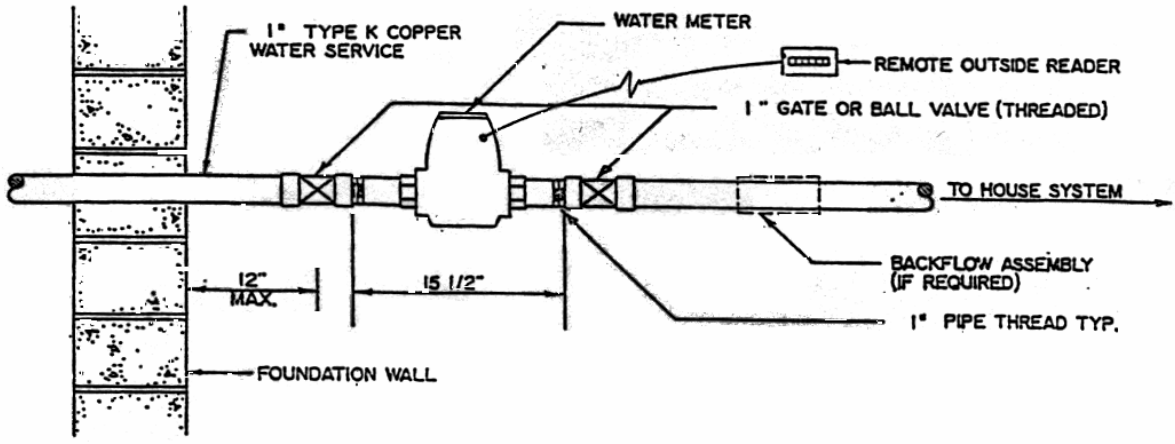
WATER SERVICE THROUGH WALL NO SCALE
