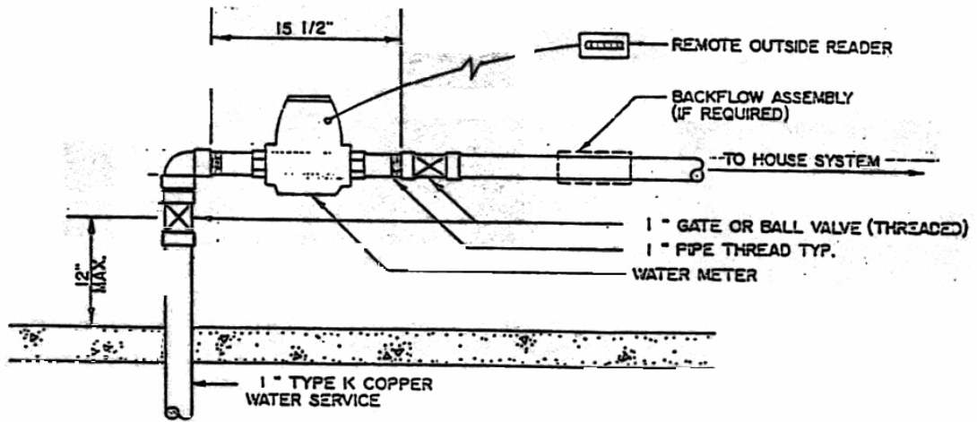
WATER SERVICE THROUGH FLOOR NO SCALE
